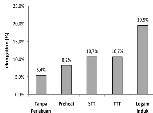
Gambar 13. Diagram perbandingan % elongation .
