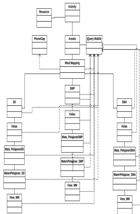
Gambar 6. Class diagram
